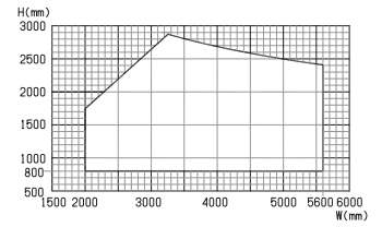
2-2 Leaves 850 Pa
