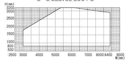
3 - 3 Leaves 850 Pa
