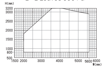
2-2 Leaves 850 Pa
