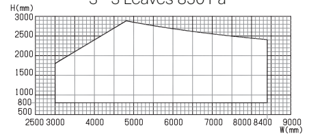
3 - 3 Leaves 850 Pa
