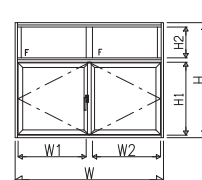
OUTSIDE VIEW
