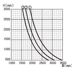
Glass groove 14mm & 24mm
