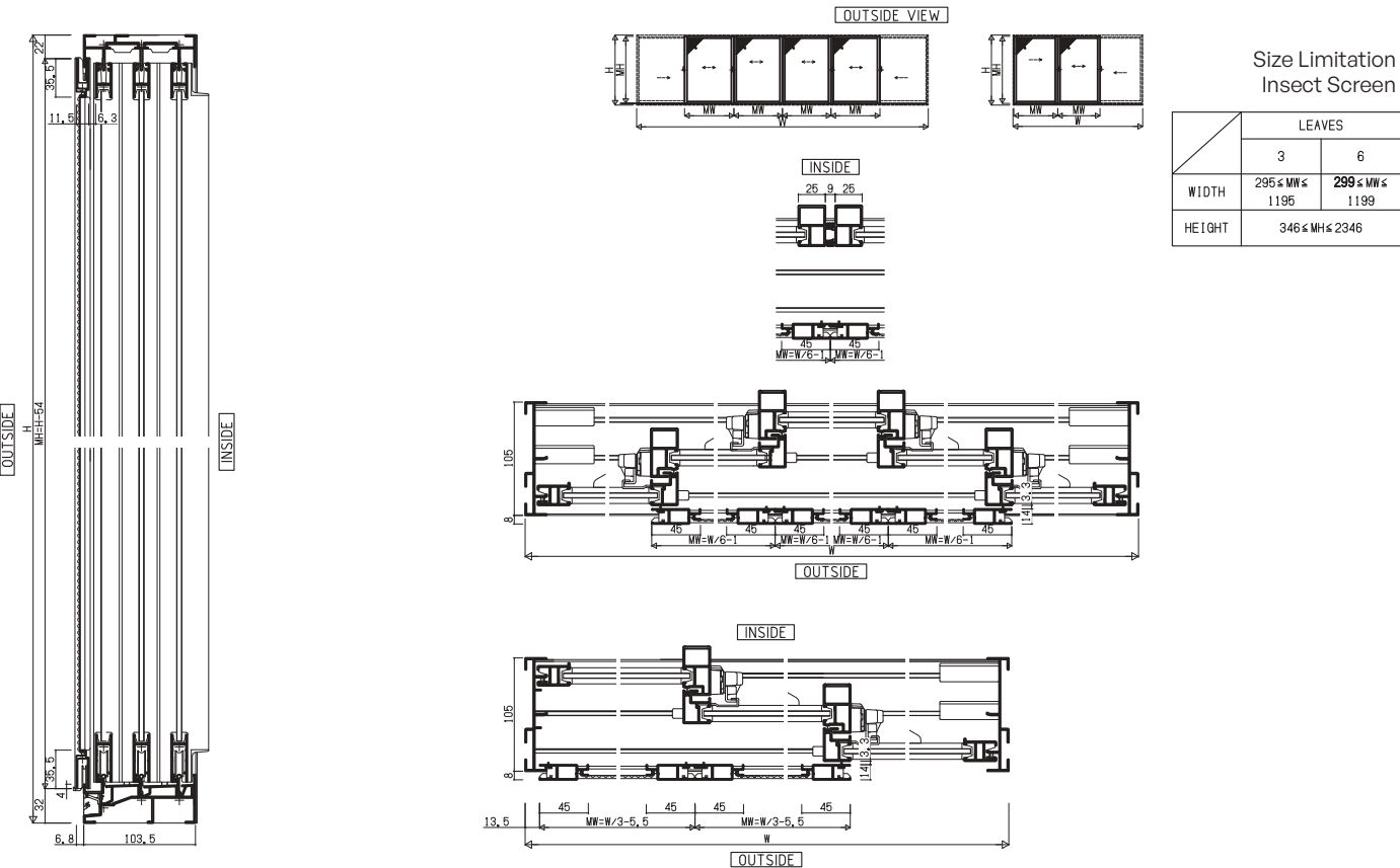
Insect Screen AN - Type 3 & 6 Leaves
