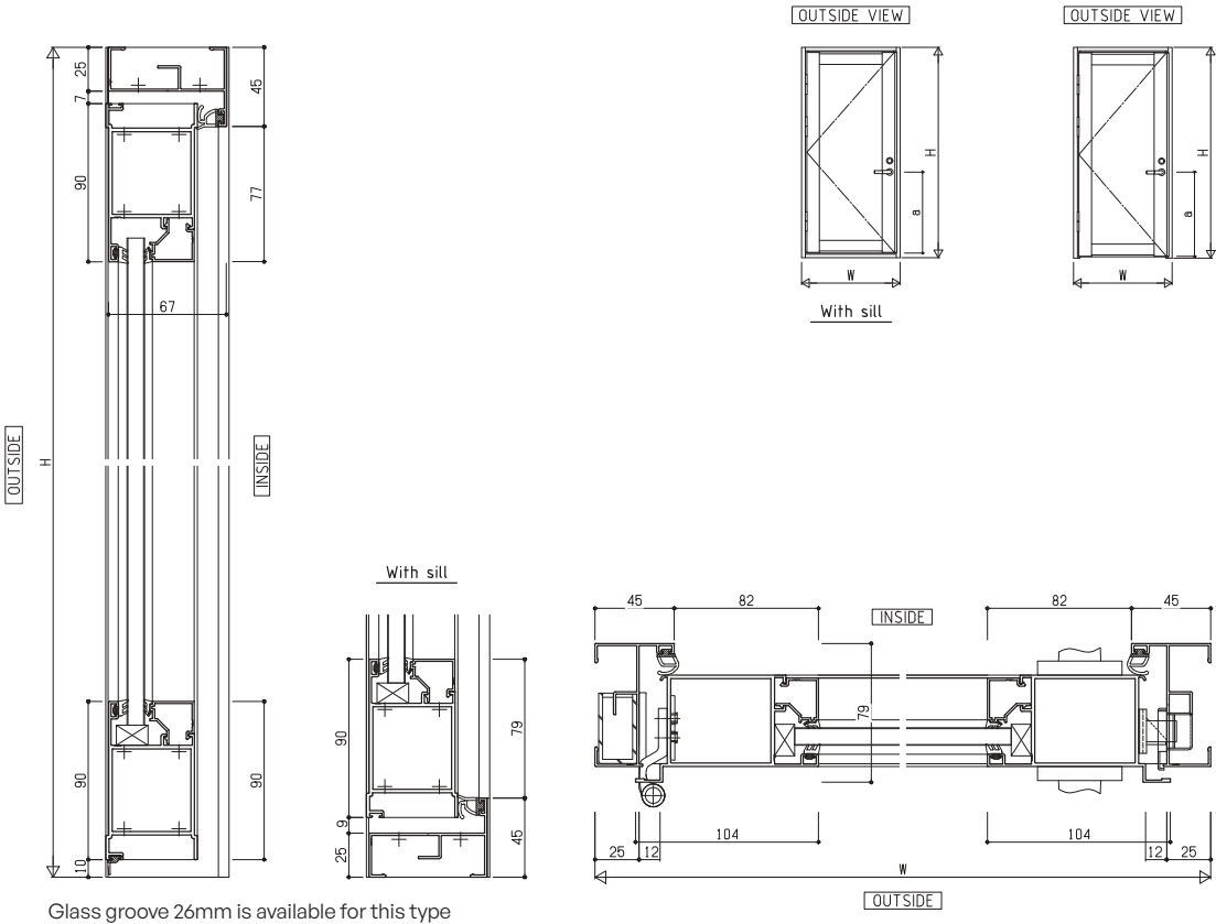
DT = 52 Outswing Single
