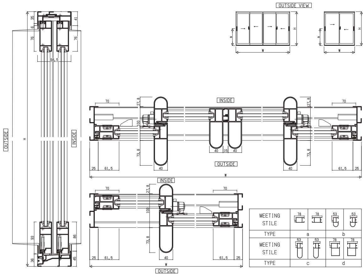
SE - Type 2 & 4 Leaves
