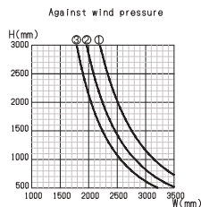
Transom 65 Glass groove 14mm
