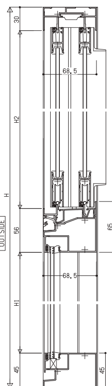
OUTSIDE VIEW
