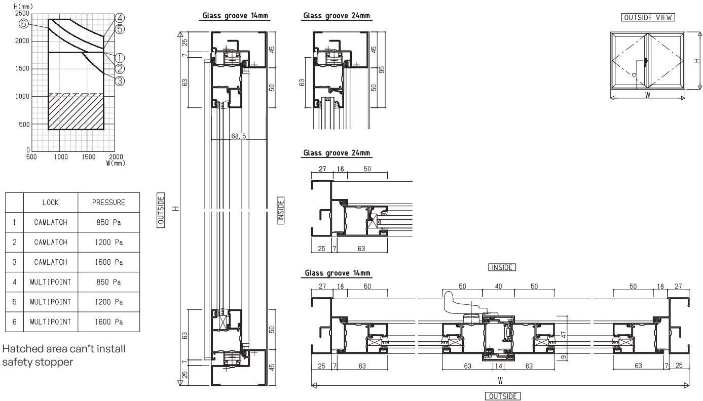
B Type Camlatch & Multipoint Double (Single Handle)
