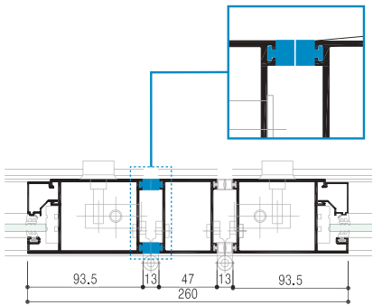
Lock Position
