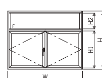
OUTSIDE VIEW
