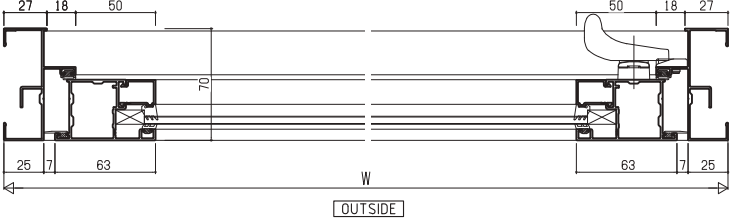
Glass groove 14mm
