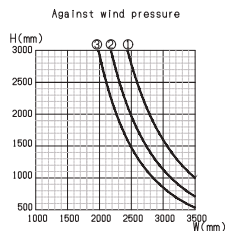
Transom 100 Glass groove 14mm
