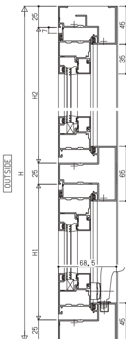
Glass groove 14mm & 24mm
