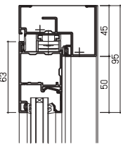
Glass groove 24mm
