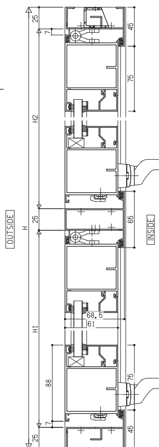
Glass groove 18mm & 26mm
