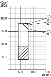
A - Type Double
