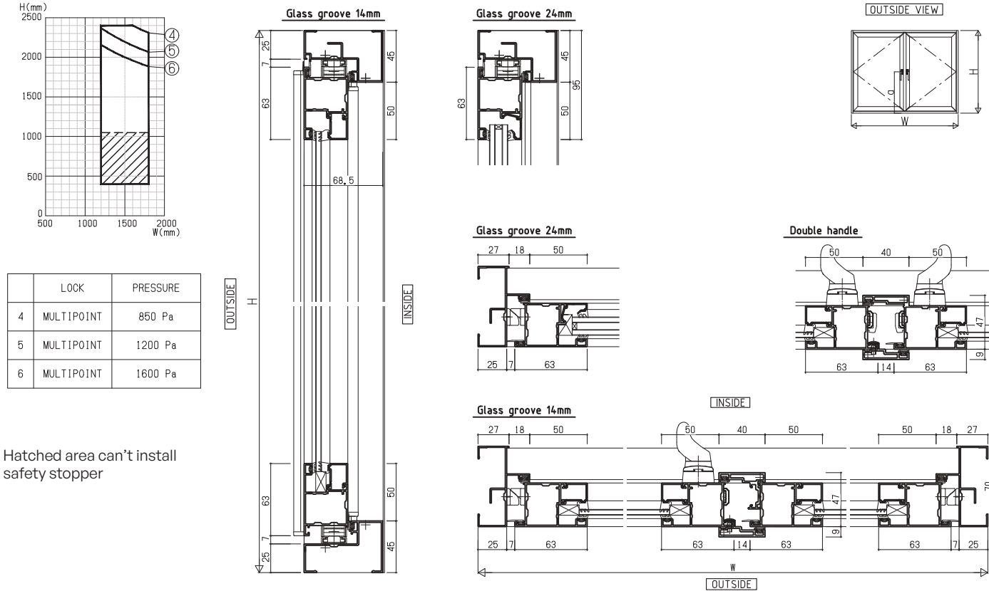
B Type Multipoint Double (Double Handle)
