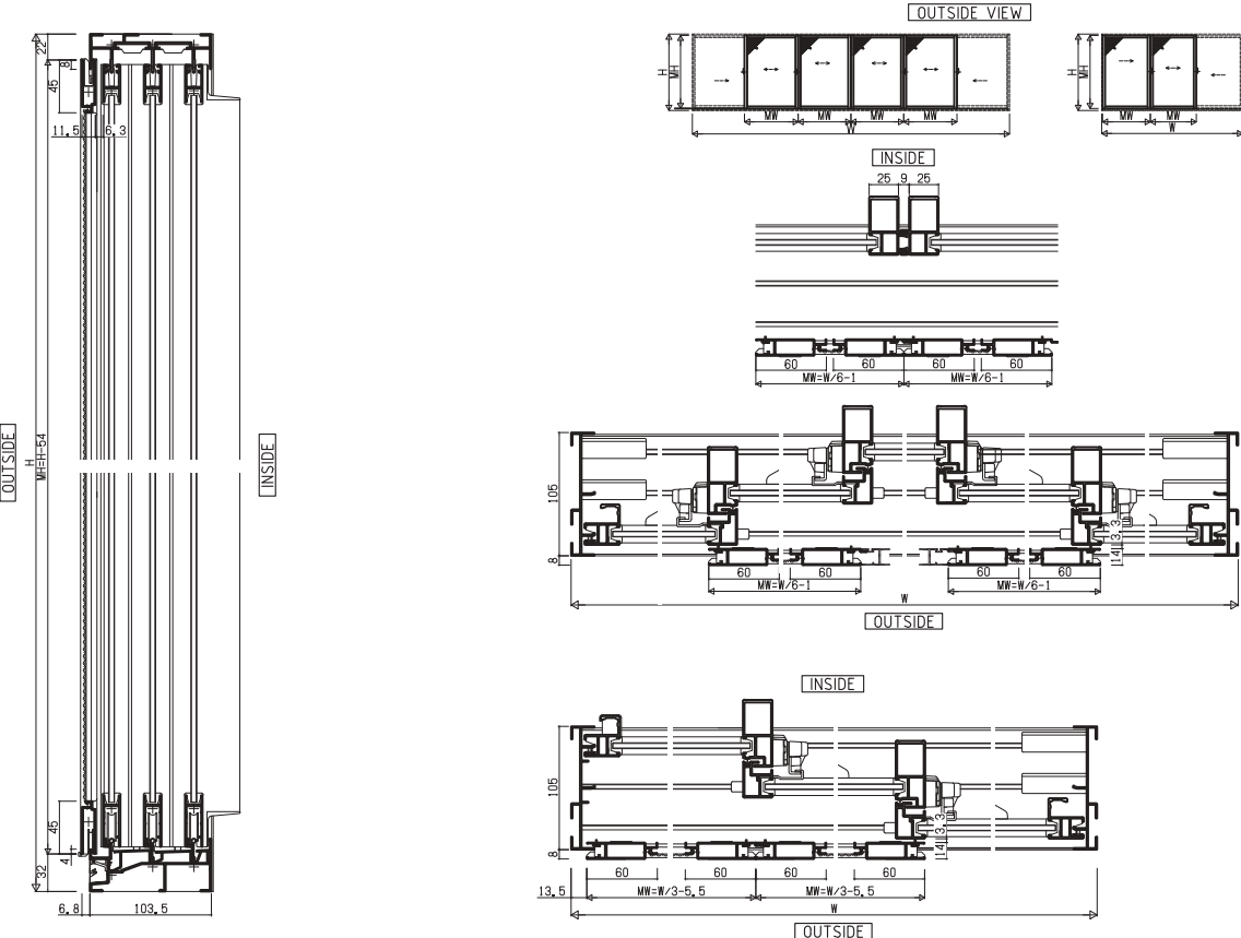
Insect Screen BN - Type 3 & 6 Leaves
