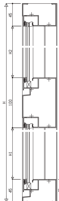
Transom 100 Glass groove 14mm
