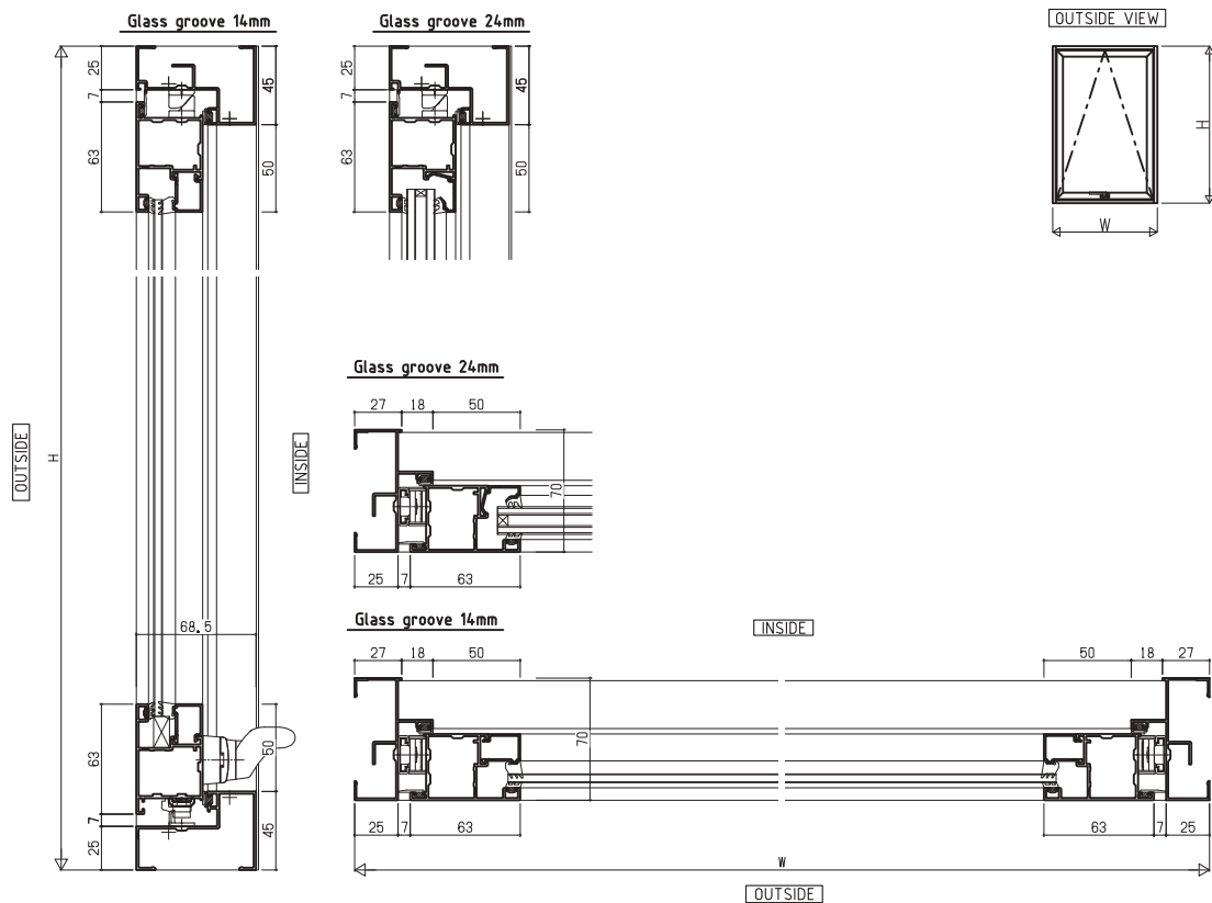
B Type - Multipoint
