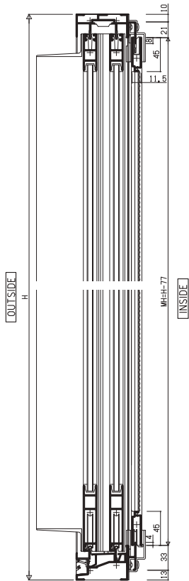
Insect Screen CF - Type 2 & 4 Leaves
