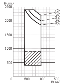
B Type - Multipoint Single
