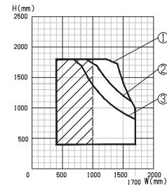
B - Type Camlatch
