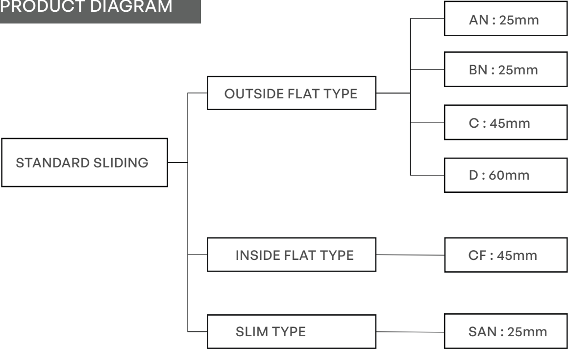
Regarding Stile Name
