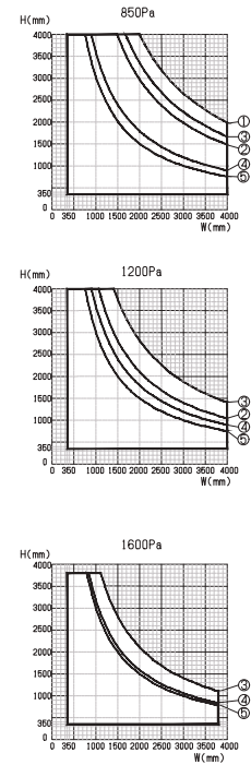
FIX square glass groove 24 mm
