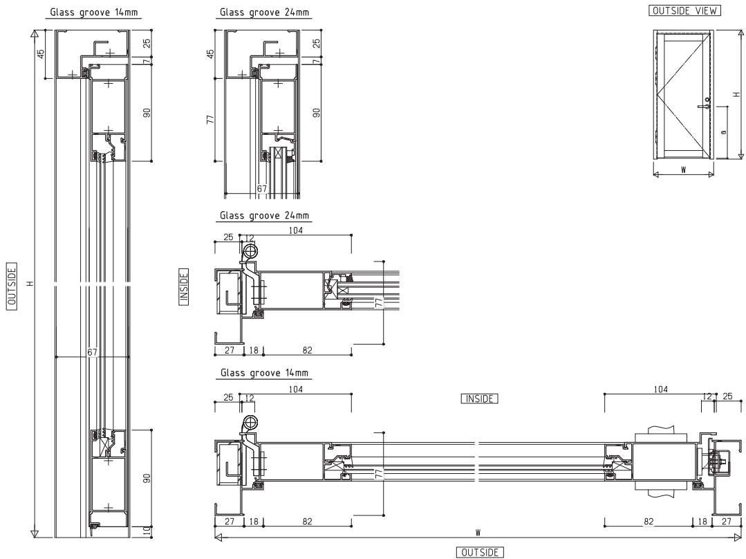
DT = 36 Outwing Single
