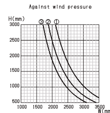
Glass groove 24mm
