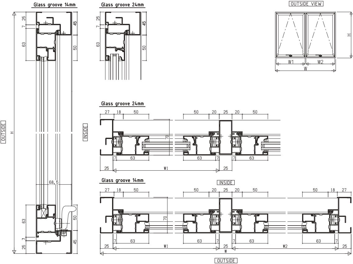
B - Type with Muntin
