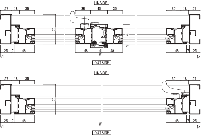
Double with single handle
